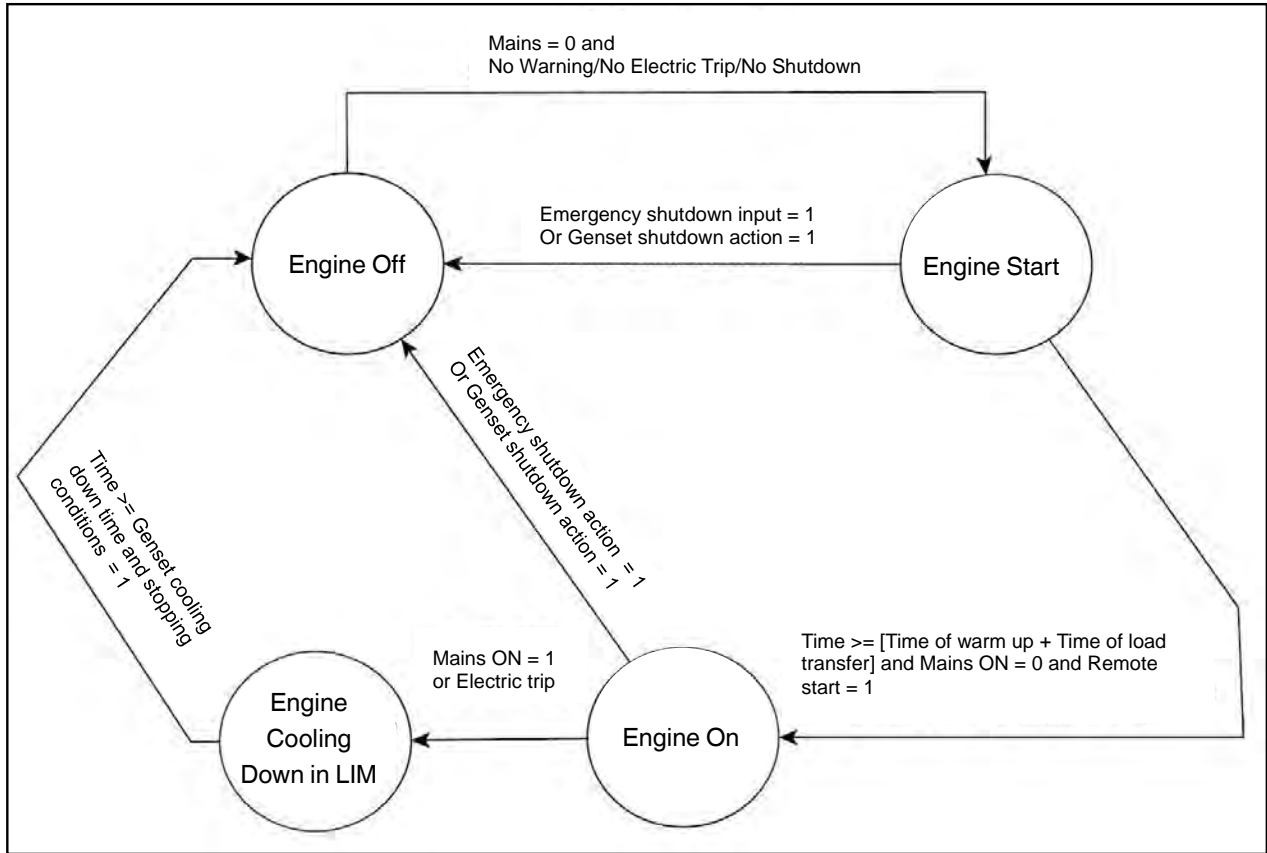
Figure 6: SMD for AMF mode
