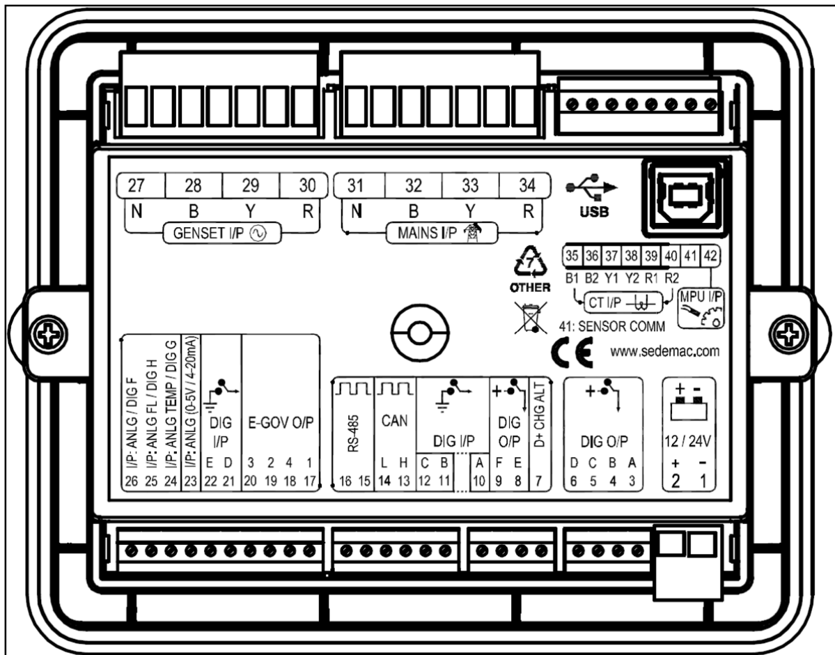
Figure 1: GC1031 Genset controller from the backside
