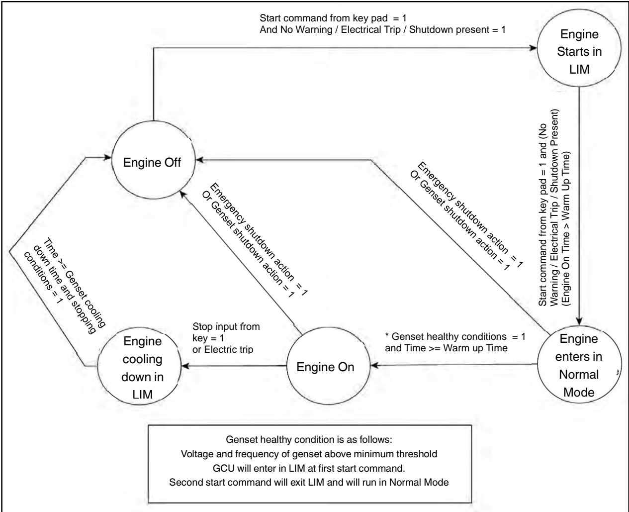
Figure 8: SMD for manual mode
